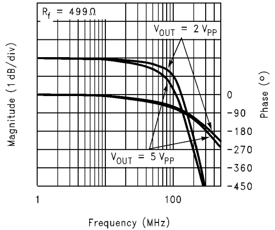
Frequency Response A_V = +6V/V
