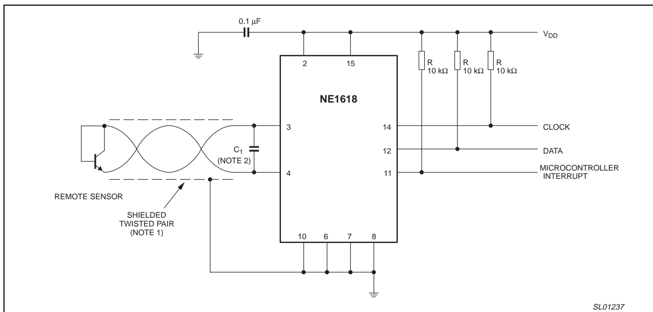
Figure 3. Typical operating circuit.
