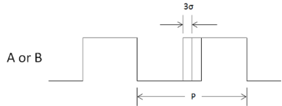
Figure 29: ABZ Jitter
