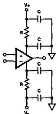
FIGURE 33. IMPROVED DECOUPLING/CURRENT LIMITING
