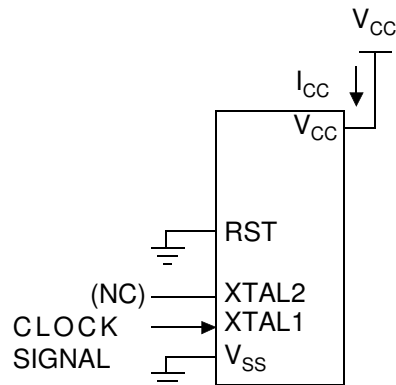
Figure 38. I_{CC} Test Condition, under reset
