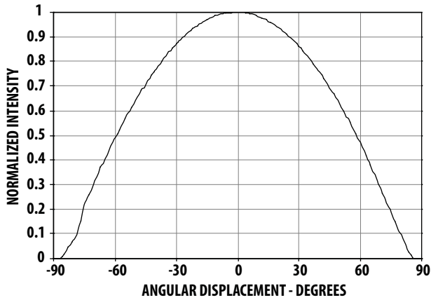
Figure 6. Radiation pattern.
