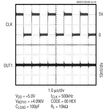
CLOCK FEEDTHROUGH
