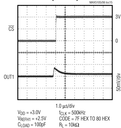
1LSB DIGITAL STEP-CHANGE (POSITIVE)
