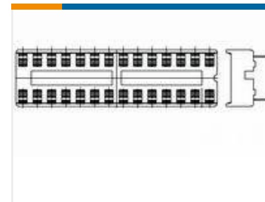
TE Part #1-2199298-5 18P,DIP SKT,300 CL,LDR,PB FREE
