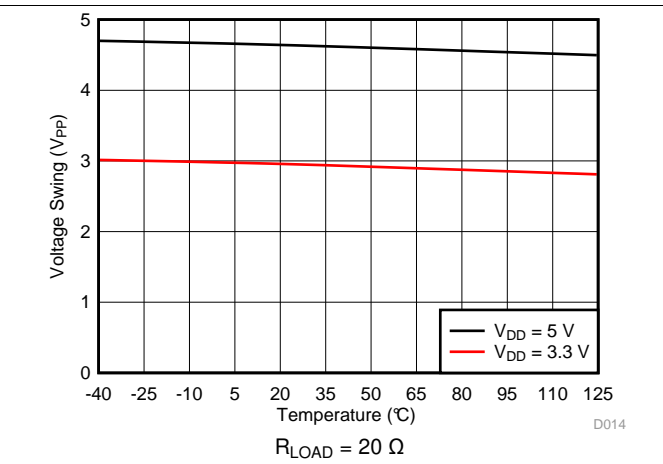
Figure 14. Positive Voltage Swing at ICOMPx Pins vs Temperature
