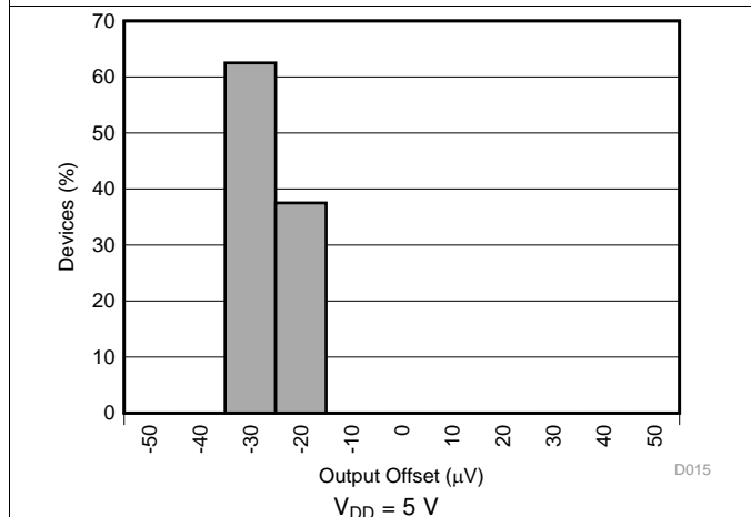
Figure 15. Shunt Sense Amplifier Offset Histogram
