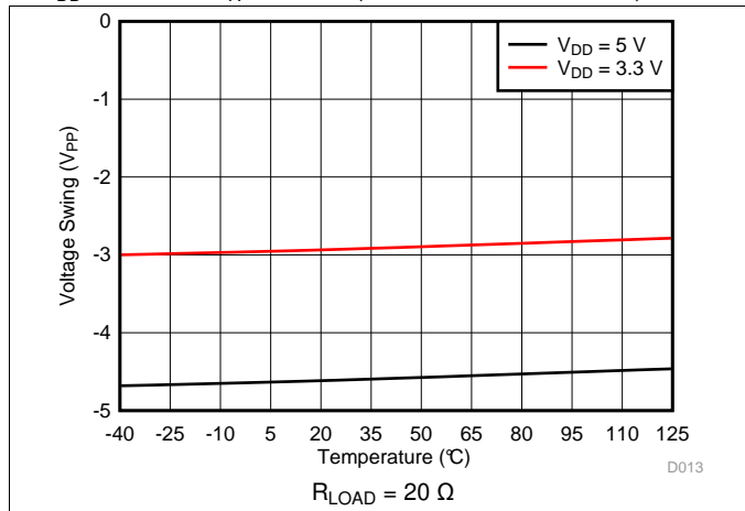
Figure 13. Negative Voltage Swing at ICOMPx Pins vs Temperature
