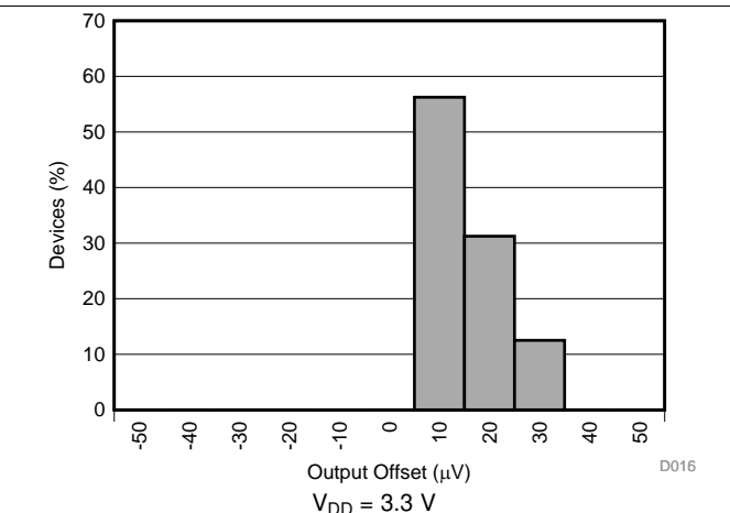
Figure 16. Shunt Sense Amplifier Offset Histogram
