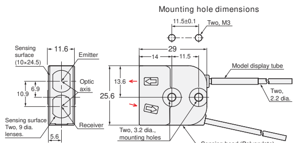
(21-F) E32-L15 2M (Free Cutting)
