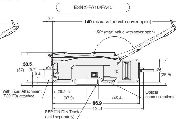
Mounted to DIN Track
