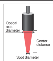
<Map of Spot Diameters and Center Distances>
