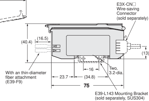
Mounting Holes
