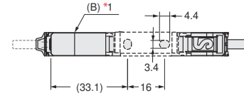
Mounting Holes
