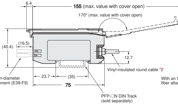
Mounted to DIN Track
