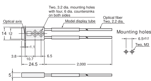
55-D E32-A12 2M (Free Cutting)
