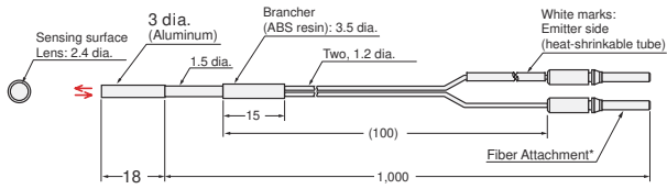
(21-E) E32-C42S 1M (No Cutting)
