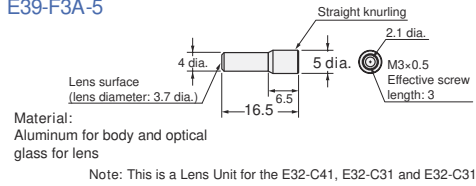
(23-C) E32-C21N 2M (Free Cutting) + E39-F3A-5
