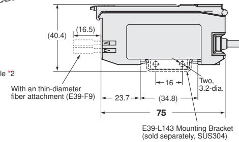
Mounting Holes
