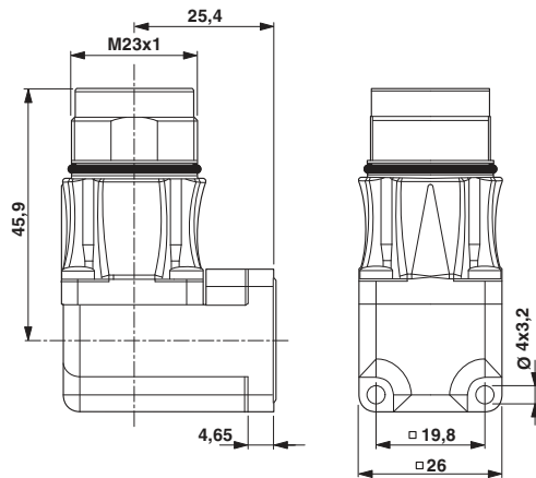
Dimensioned drawing
