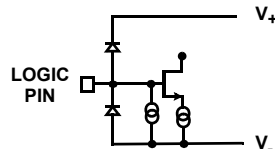
CIRCUIT 2
