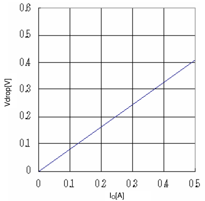
Fig.22 Minimum dropout Voltage 2 (Vcc=4.5V、Ta=25°C)
