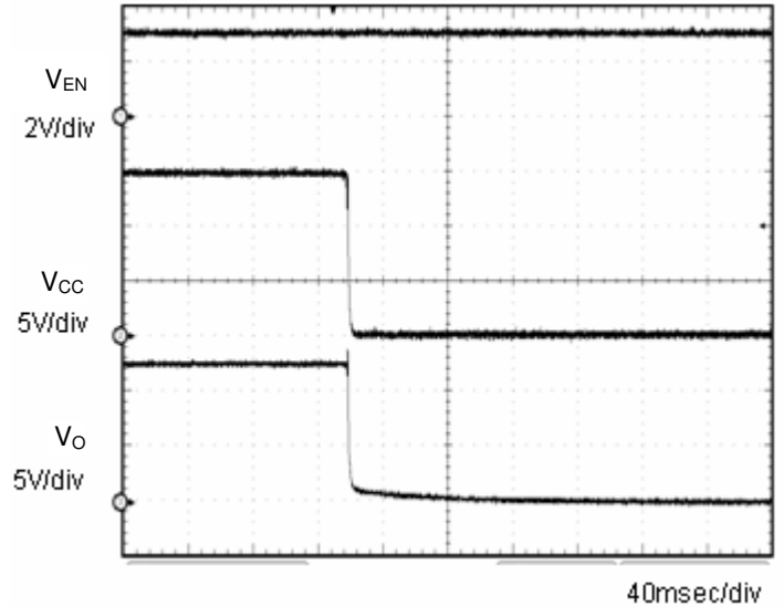
Fig.6 OFF sequence 1 Co=1μF
