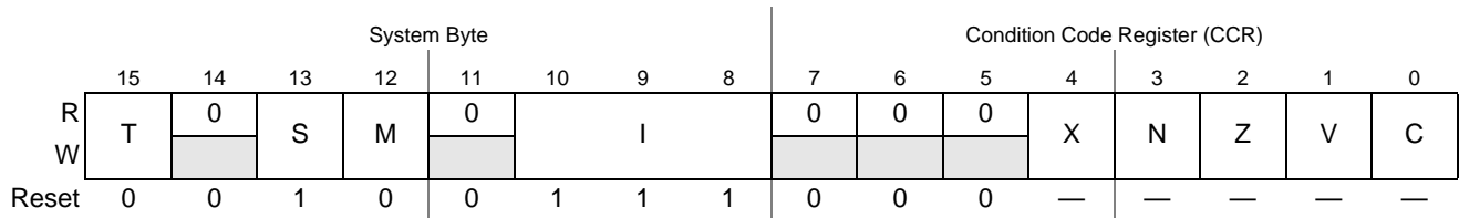
Figure 2-8. Status Register (SR)
