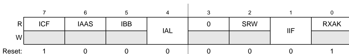
Figure 24-5. I 2 C Status Register (I2SR)
