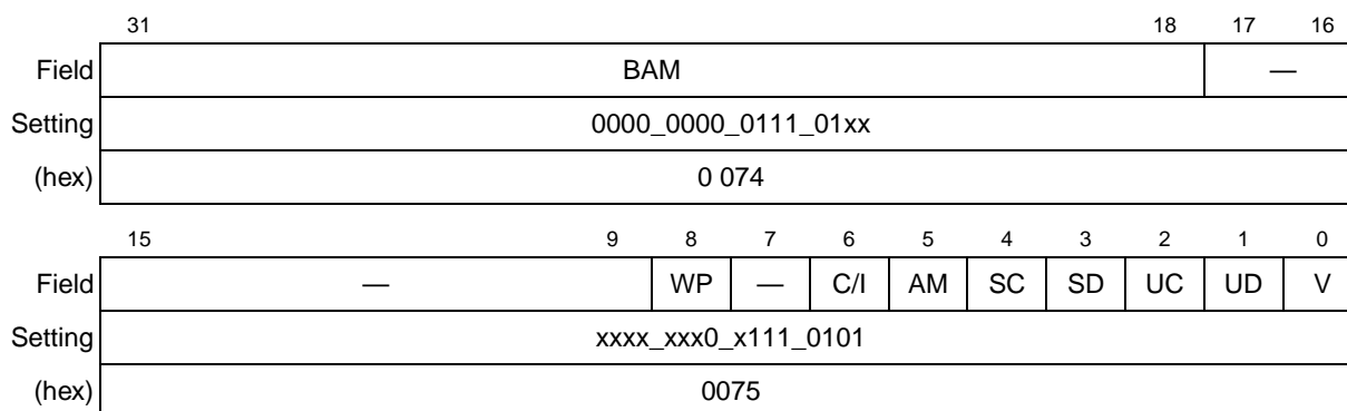
Figure 15-14. DMR0 Register
