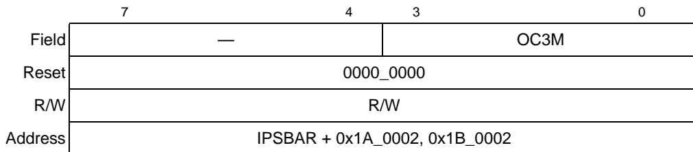
Figure 20-4. GPT Output Compare 3 Mask Register (GPTOC3M)
