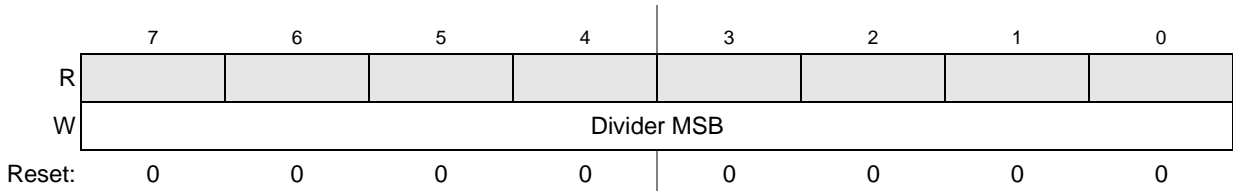
Figure 23-13. UART Baud Rate Generator Registers (UBG1 n )
