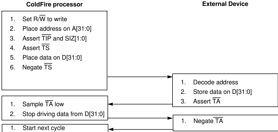
Figure 13-7. Write Cycle Flowchart
