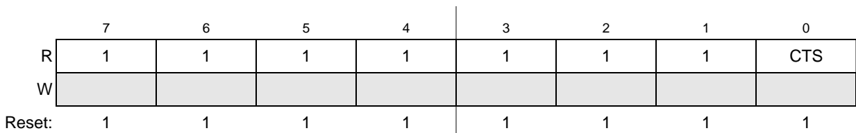
Figure 23-15. UART Input Port Registers (UIP n )
