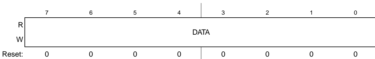
Figure 24-6. I 2 C Data I/O Register (I2DR)
