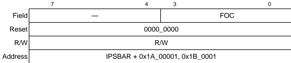
Figure 20-3. GPT Input Compare Force Register (GPCFORC)
