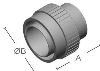
HD/HDP Plug
