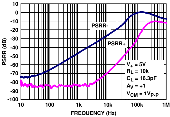
FIGURE 11. PSRR vs FREQUENCY, V_+ = 5V, V_- = \pm 1.2V
