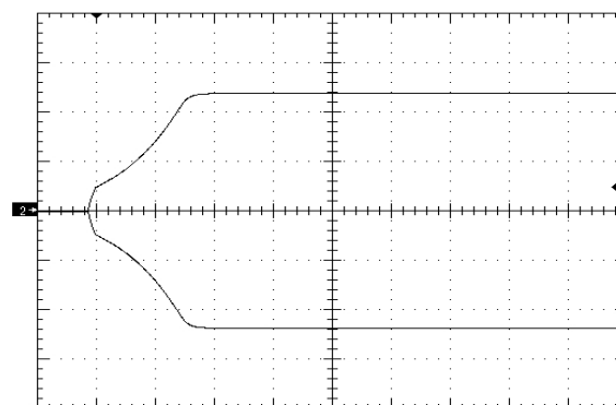
Figure 9. Startup Waveform via Input Voltage, time scale 10mS/div. Vin=Vin_nom, Iout=full load Cout=10uF, Ch1=+Vout (5V/div), Ch2=-Vout (5V/div)
