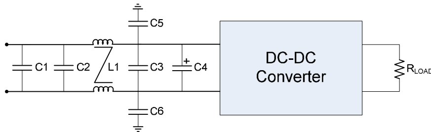
Figure 13. EMI Filter
