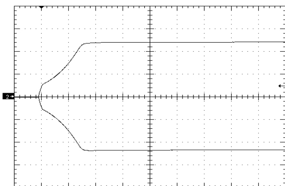
Figure 8. Startup Waveform via Enable Pin, time scale 10mS/div. Vin=Vin_nom, Iout=no load Cout=0, Ch1=+Vout (5V/div), Ch2=-Vout (5V/div)
