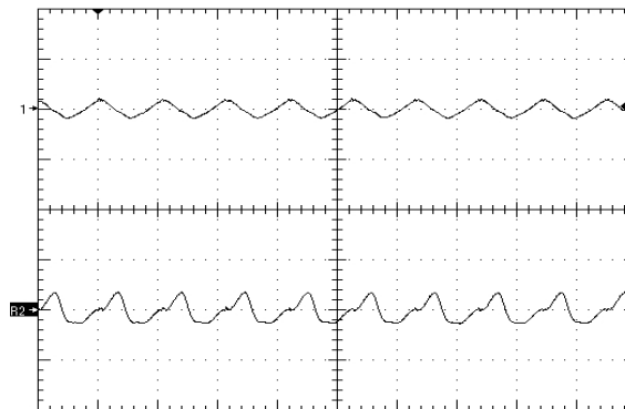
Figure 7. Output Voltage Ripple (50mV/div), time scale – 2uS/div. Vin=Vin_nom, full load Cout=0.1uF ceramic + 10uF Tantalum (see Fig 16)
