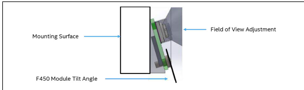
Figure 3-5: System Tilt
