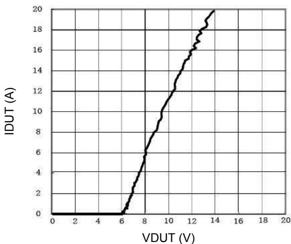
Figure 5. Transmission Line Pulse ( t_p=100\text{ns} )
