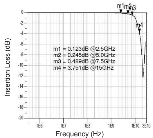
Figure 4. Insertion Loss S21 - I/O to I/O
