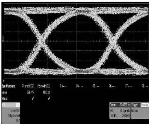
Figure 3. Eye Diagram - USB3.1 at 10Gbps per Channel (with GSCLAMP3324PE)
