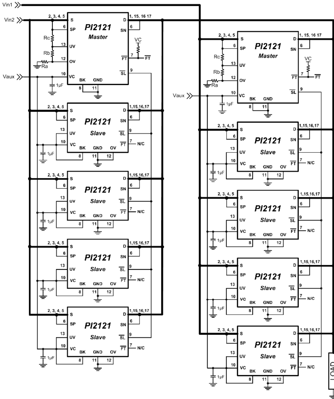
Figure 23: PI2121 used in a 100A Active ORing application (master/slave configuration)
