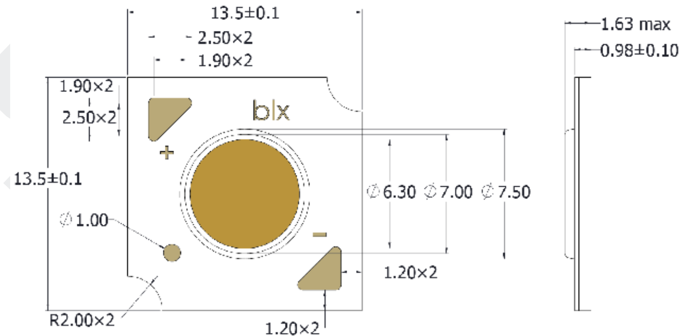
Figure 19: V6 HD LED Array
