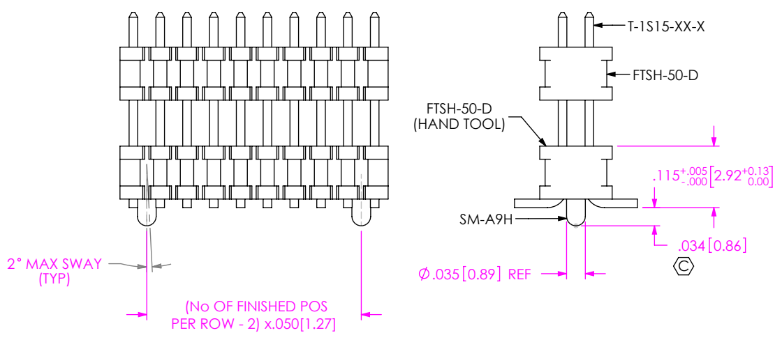
FIG 8 -A OPTION (STAKED) 6 POSITION MIN DIFFERENT AS SHOWN OTHERWISE SAME AS FIG 1
