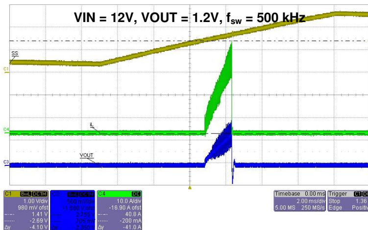
Fig. 8 Hiccup Mode Over Current Protection (C1: SS1, C4: I_{out} , C3: VOUT)
