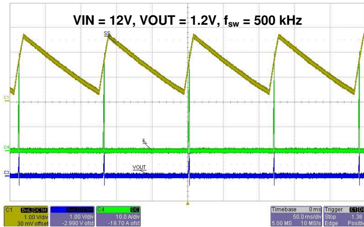
Fig. 7 Hiccup Mode Over Current Protection (C1: SS1, C4: I_{out} , C3: VOUT)
