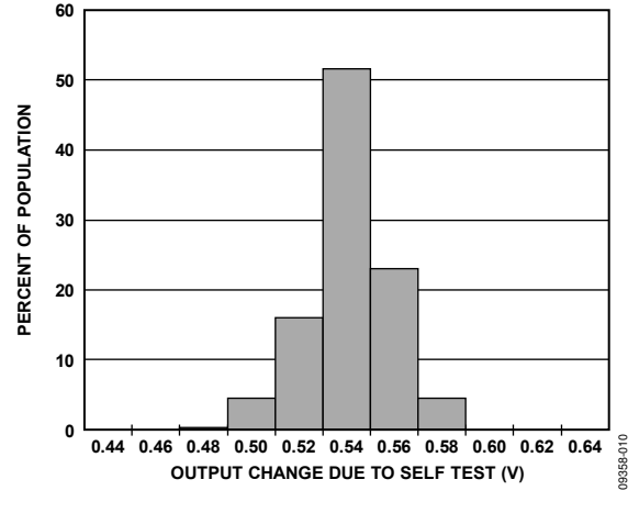
Figure 8. Z-Axis Self-Test Response at 25°C, V_s = 3 V
