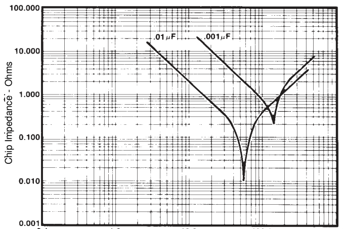
Impedance vs. Frequency for Ceramic Capacitors—C0G Dielectric
