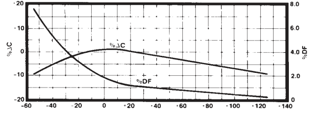
Capacitance & DF vs. Temperature-X7R
