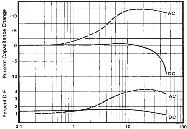
AC or DC Volts Applied Typical Effect of 1000 Hz AC and DC Voltage Level on Capacitance and Dissipation Factor — X7R Note: C0G Dielectric capacitance and dissipation factor are stable with voltage.
