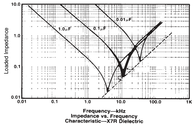
Impedance vs. Frequency For Ceramic Capacitors — X7R Dielectric
