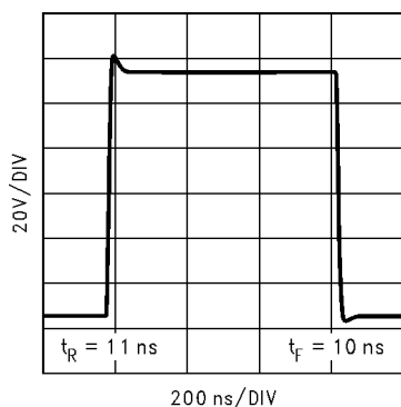
FIGURE 5. LM2426 Pulse Response
