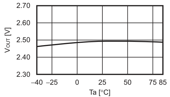
5.2 V_{OUT} = 2.5 V
