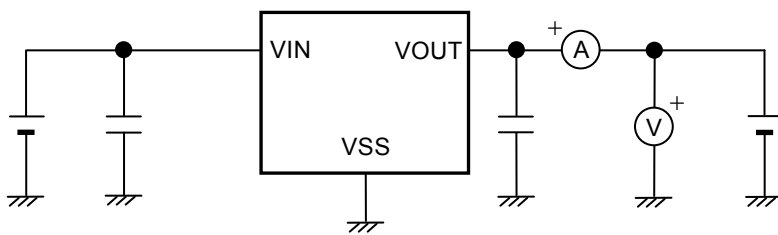
Figure 6 Test Circuit 3
