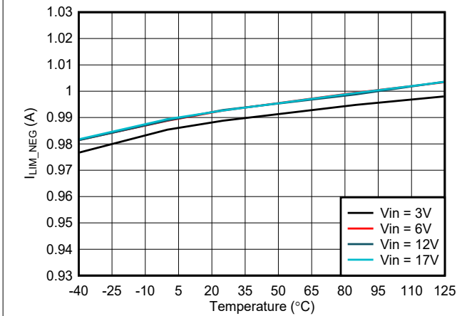
Figure 7-15. Low-Side I_{NEG} vs Temperature
