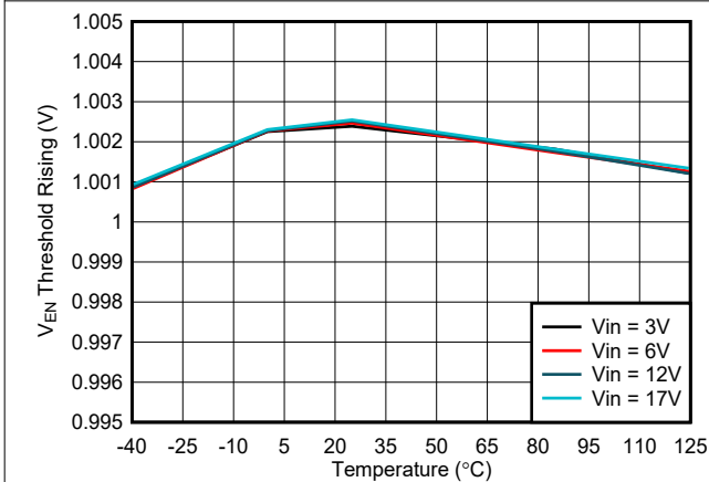
Figure 7-17. Precision Enable Threshold vs Temperature
