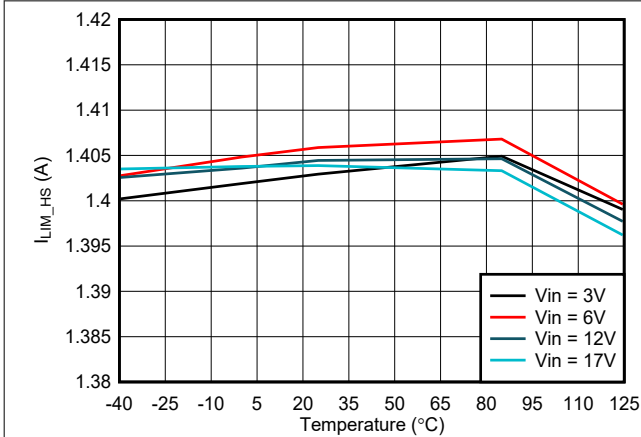
Figure 7-13. High-Side I_{LIM} vs Temperature
