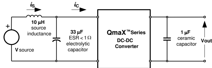
Fig. 1.5V.11: Test Setup for measuring input reflected ripple currents, i_c and i_s .
