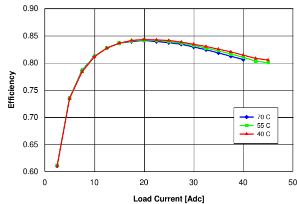
Fig. 1.0V.4: Efficiency vs. load current and ambient temperature for converter mounted vertically with V_{in} = 48\text{ V} and air flowing from pin 3 to pin 1 at a rate of 200 LFM (1.0 m/s).
