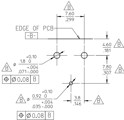
RECOMMENDED PCB PATTECPN
