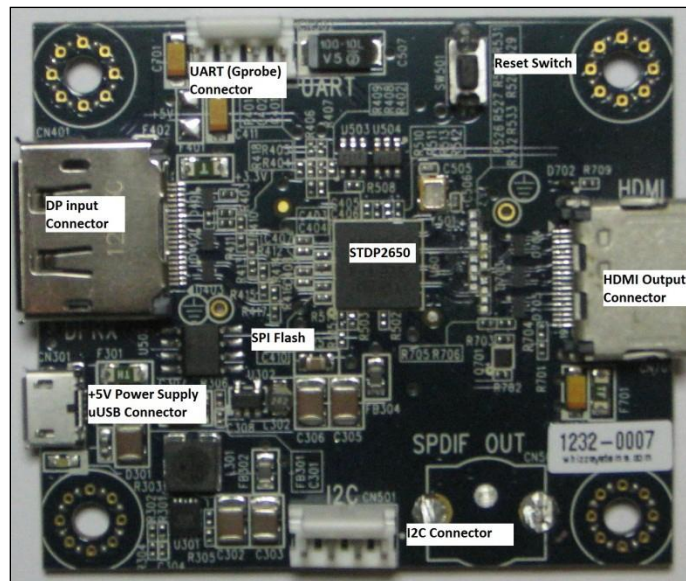
Figure 1. Board Picture
