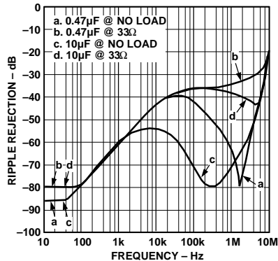
Figure 18. Power Supply Ripple Rejection on ADP3302AR3
