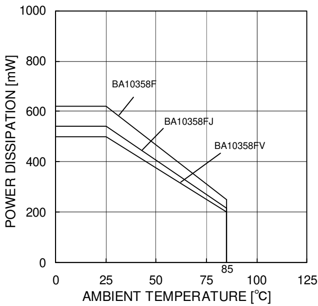
Figure 2. Derating Curve
