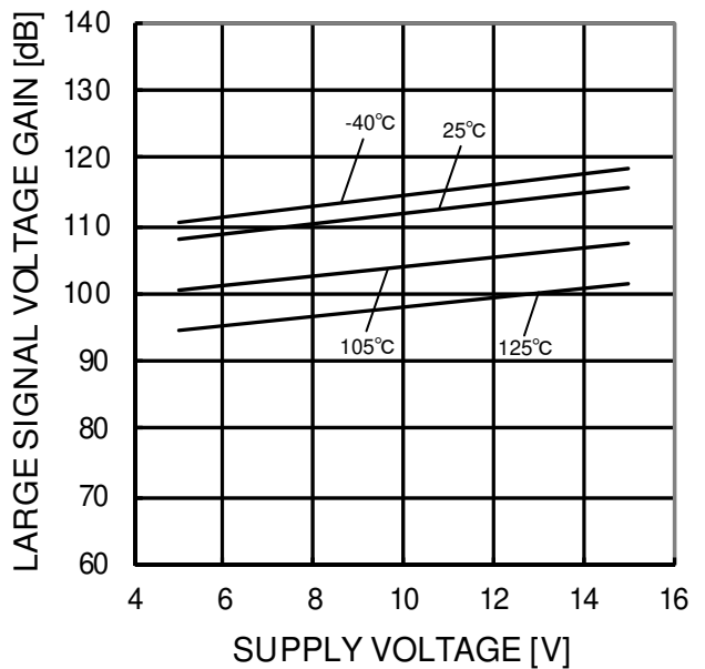
Figure 93. Large Signal Voltage Gain - Supply Voltage ( R_L=2k\Omega )
