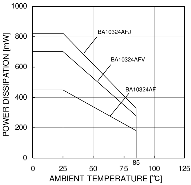
Figure 26. Derating Curve
