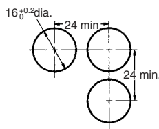
Square A16□-A/M16□-A, A165□-BA, M165-BA Round A16□-T/M16□-T (Top View)
