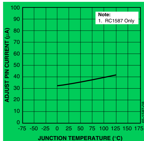
Figure 6. Adjust Pin Current vs. Temperature
