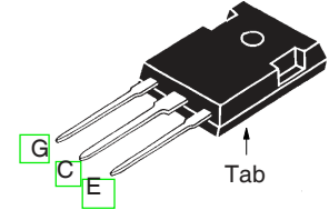
TO-247 AD
