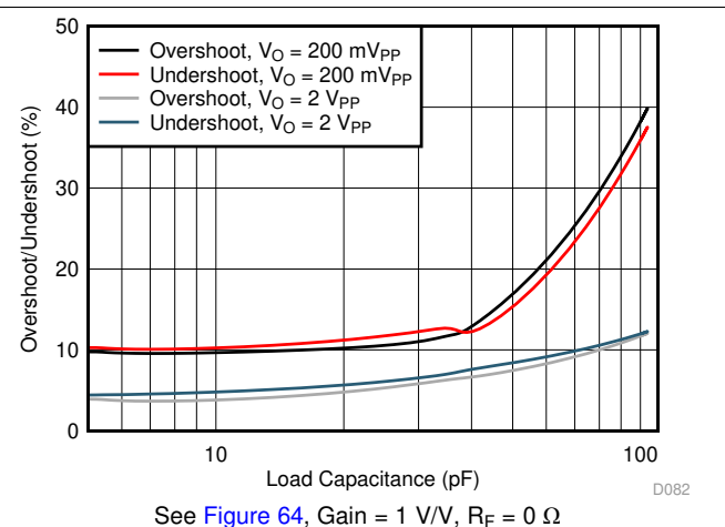
Figure 30. Overshoot and Undershoot vs C_L
