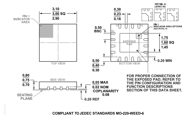
Figure 41. 16-Lead Lead Frame Chip Scale Package [LFCSP] 3 mm × 3 mm Body and 0.75 mm Package Height (CP-16-22) Dimensions shown in millimeter
