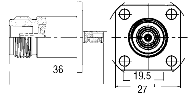
Type N Female 4-Hole Flange 3190-2213
