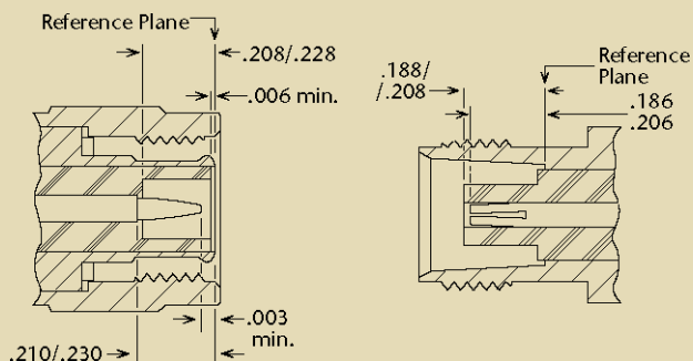
Plug (male)
