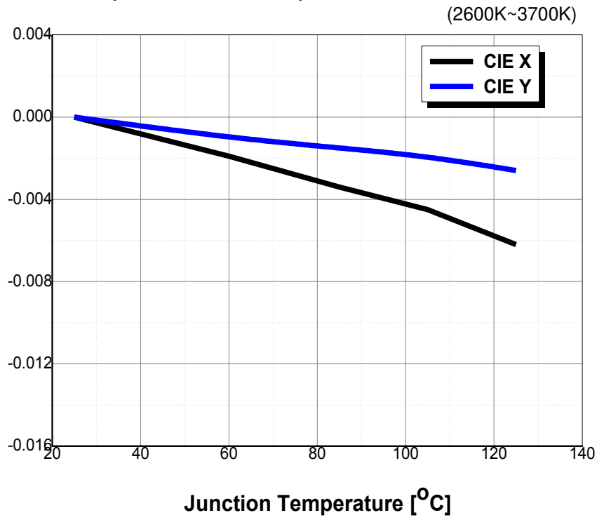
Fig 8. Junction Temp. vs. CIE X, Y Shift, I_F=750\text{mA}
