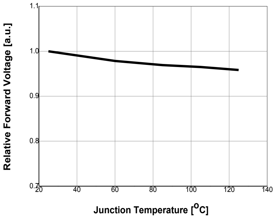
Fig 7. Relative Forward Voltage vs. Junction Temperature, I_F=750\text{mA}
