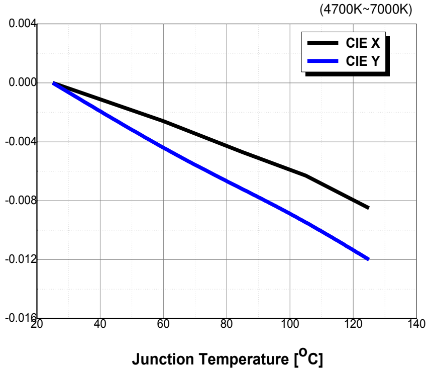
Fig 8. Junction Temp. vs. CIE X, Y Shift, I_F=750mA
