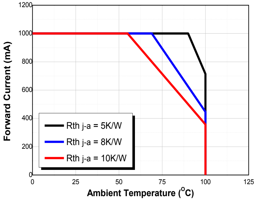
Fig 9. Maximum Forward Current vs. Ambient Temperature, T_j(\text{max.})=125^\circ\text{C} , I_F=1\text{A}
