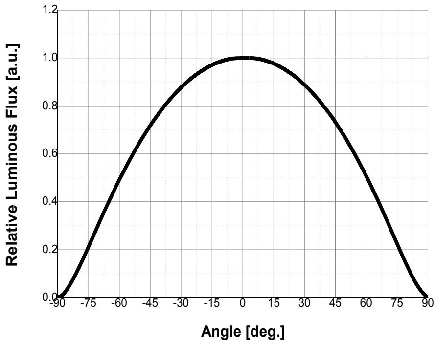
Fig 2. Radiant pattern, T_j=25^\circ\text{C} , I_F=750\text{mA}
