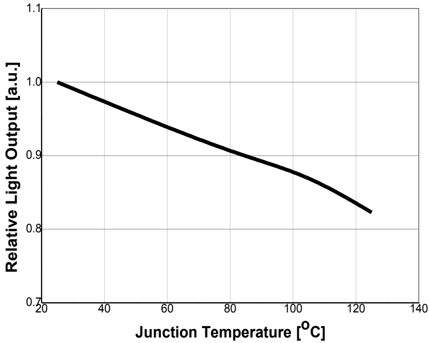
Fig 6. Relative Light Output vs. Junction Temperature, I_F=750\text{mA}
