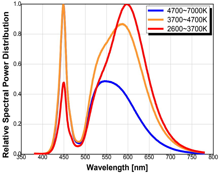
Fig 1. Color Spectrum, T_j=25^\circ\text{C} , I_F=750\text{mA}
