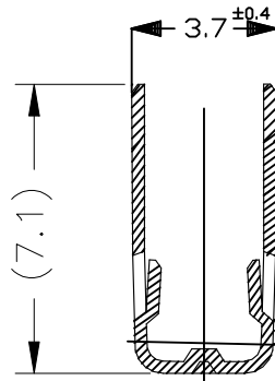
SECT B-B
