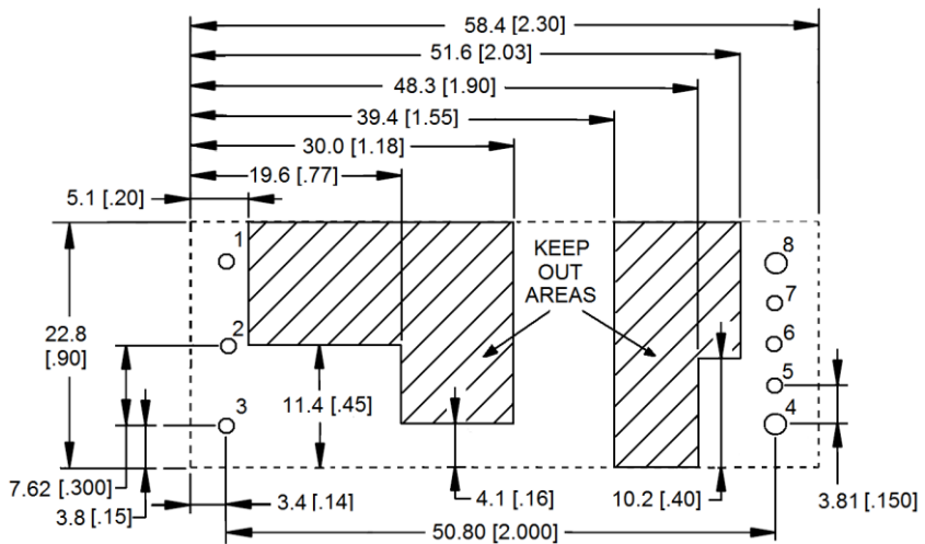
SMT Recommended Pad Layout (Component Side View)
