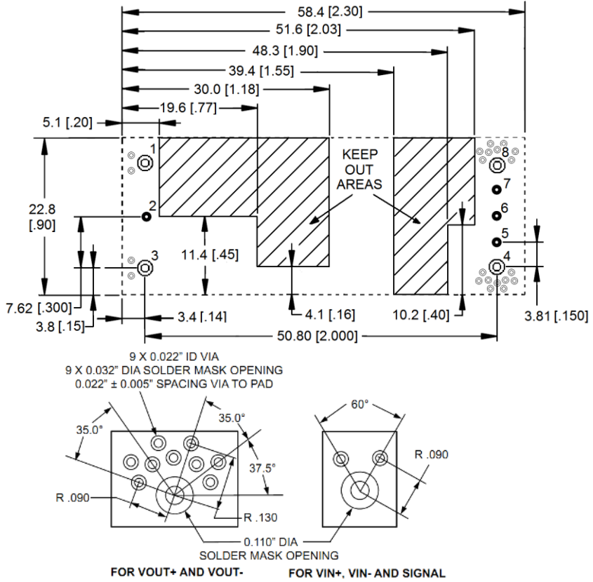
SMT Recommended Pad Layout (Component Side View)
