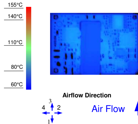
Figure 8. Thermal Image for Airflow Direction 3 (4A output, 55°C ambient, 200 LFM, typical Vin, open frame, unit soldered onto a fixture board)
