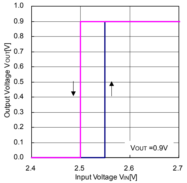
Figure 20. V_{IN} start up
