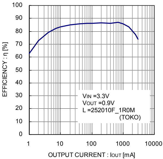
Figure 21. Efficiency
