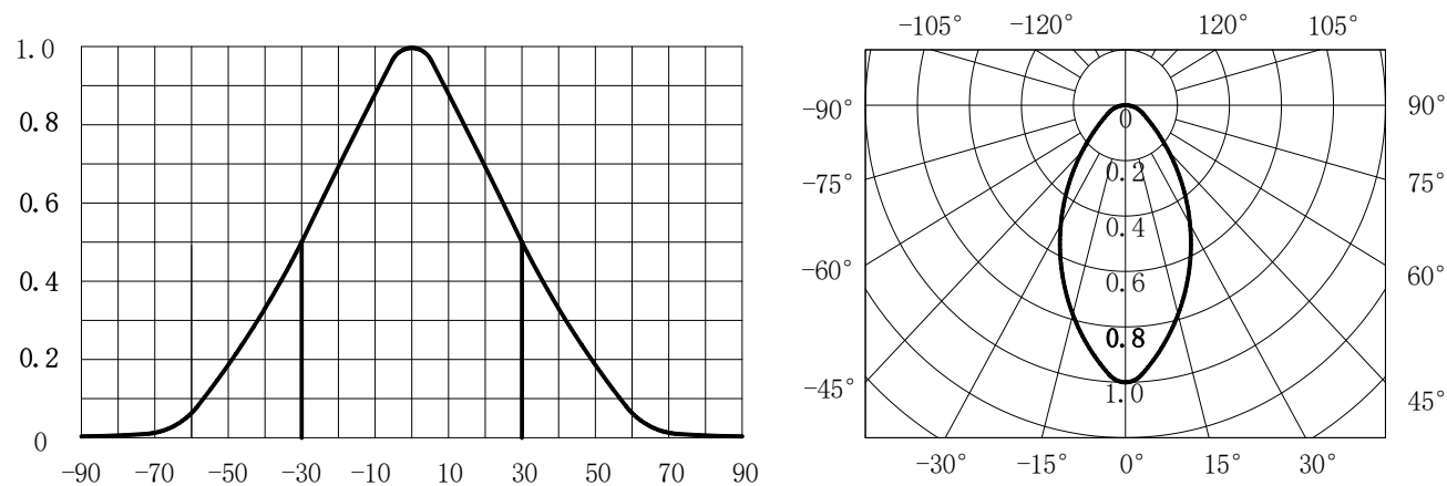
配光曲线 Light distribution curve
