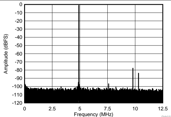
SFDR = 77 dBc, SNR = 68.2 dBFS, SINAD = 67.7 dBFS, THD = 75 dBc, HD2 = 77 dBc, HD3 = 83 dBc
