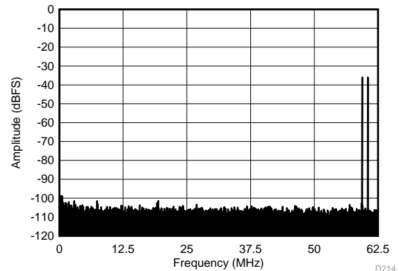
f_{IN1} = 185\text{ MHz} , f_{IN2} = 190\text{ MHz} , \text{IMD3} = 102\text{ dBFS} , each tone at -36\text{ dBFS}
