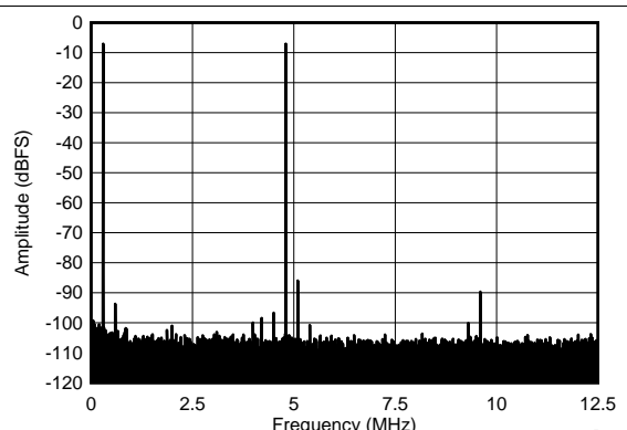
f_{IN1} = 46 \text{ MHz} , f_{IN2} = 50 \text{ MHz} , IMD3 = 90, each tone at = -7 dBFS
