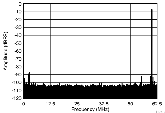
f_{IN1} = 185\text{ MHz} , f_{IN2} = 190\text{ MHz} , \text{IMD3} = 86\text{ dBFS} , each tone at -7\text{ dBFS}
