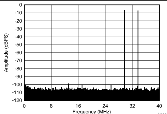
f_{IN1} = 46\text{ MHz} , f_{IN2} = 50\text{ MHz} , IMD3 = 98 dBFS, each tone at -7 dBFS
