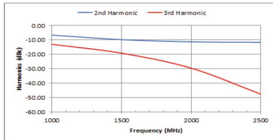
Harmonics (@ Psat)
