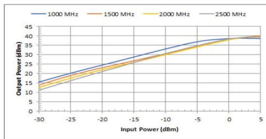
Output Power vs. Input Power
