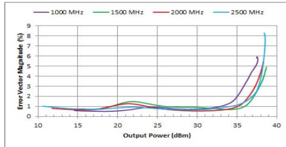
Error Vector Magnitude (%) [w/ QPSK Waveform]
