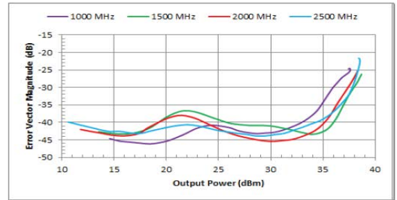
Error Vector Magnitude (dB) [w/ QPSK Waveform]
