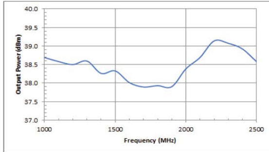
RF Output Power
