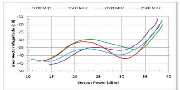
Error Vector Magnitude (dB) [w/ 16QAM Waveform]
