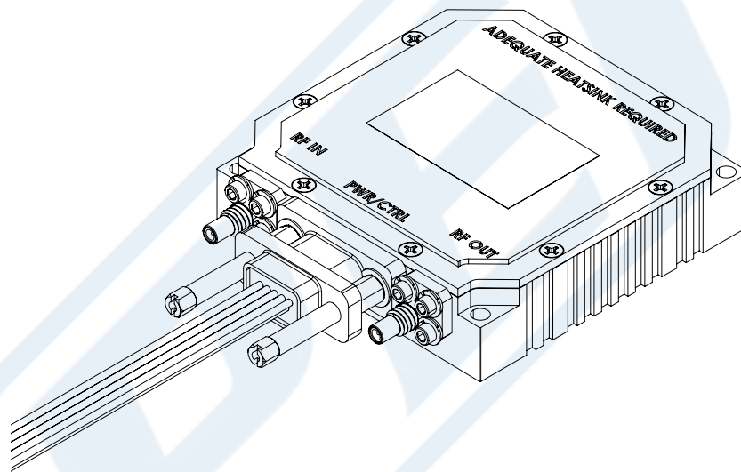
illustration of Amplifier & Interface Cable
