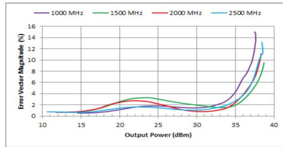
Error Vector Magnitude (%) [w/ 16QAM Waveform]
