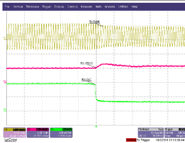
Figure 9. Start-Up with bq51013B
