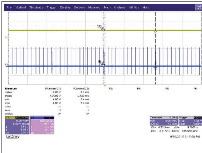
Figure 8. Standby Power
