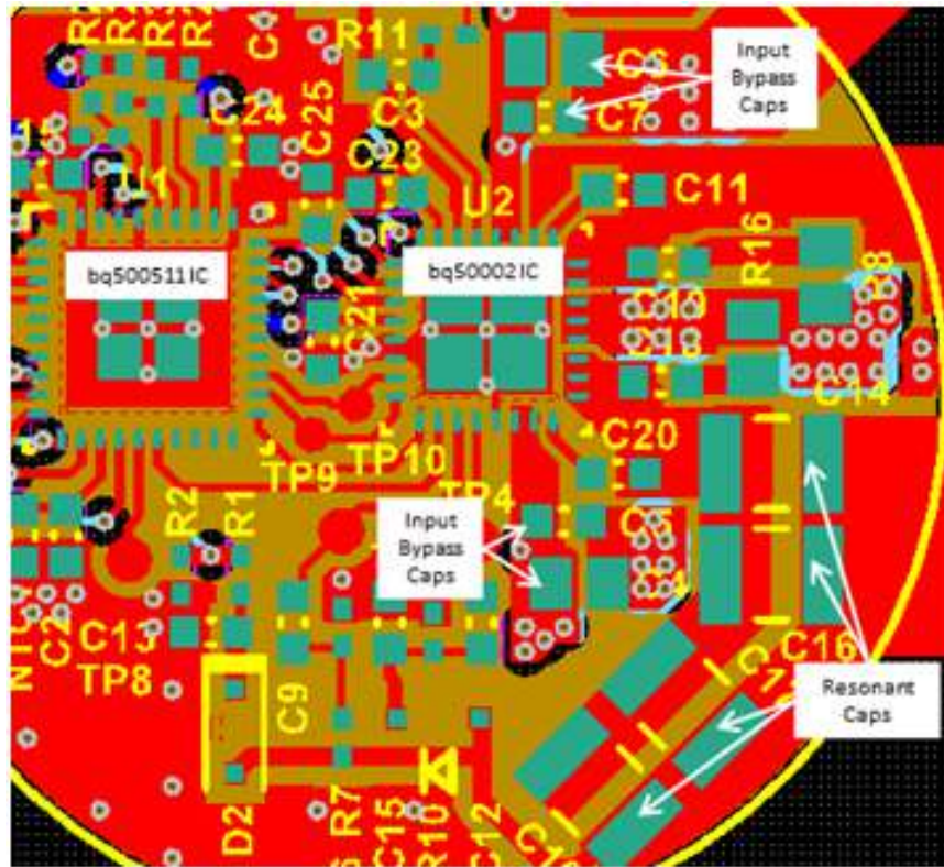
Figure 13. Ground Layout
