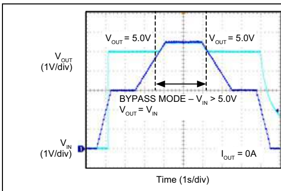
FIGURE 2-20: Bypass Mode.
