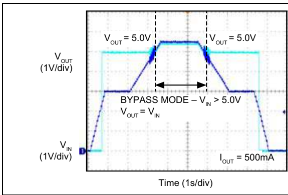
FIGURE 2-21: Bypass Mode.
