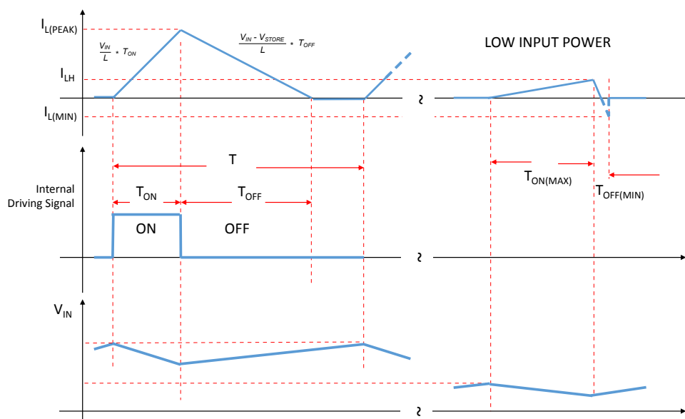
Figure 27. Inductor current and input voltage waveforms
