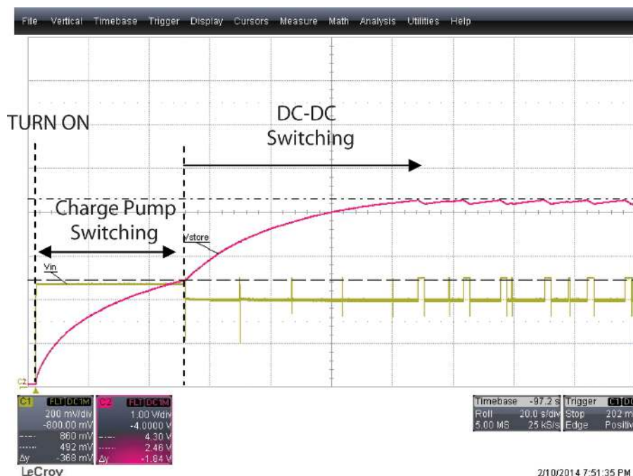
Figure 5. Boost start-up
