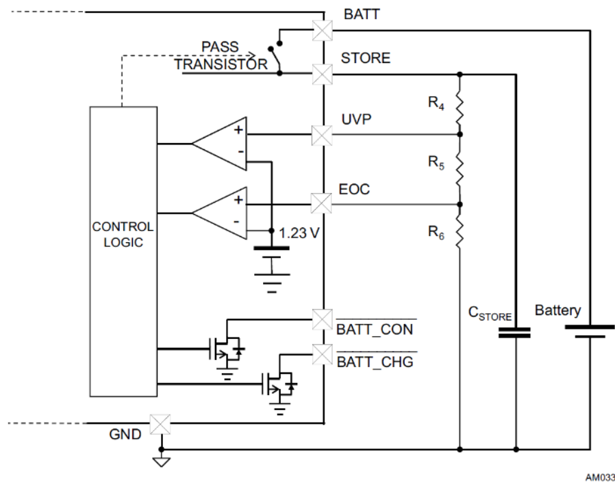
Figure 2. Battery management section
